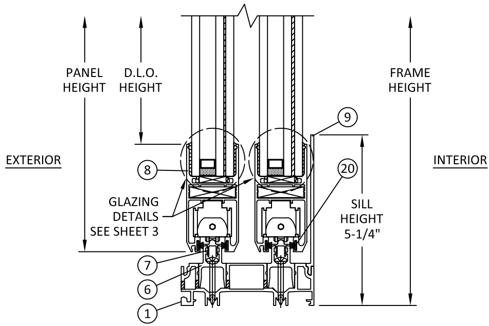
B 5 VERTICAL SECTION 2-TRACK SILL
