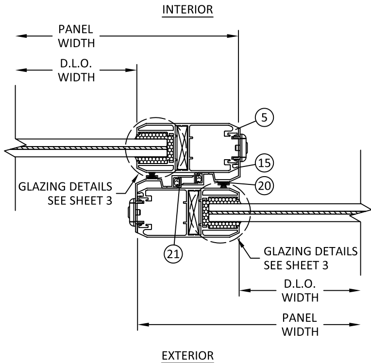
M 8 HORIZONTAL SECTION INTERLOCK
