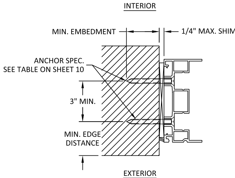
T 9 INSTALLATION DETAIL 2-TRACK JAMB
