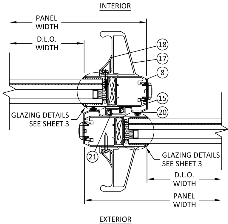
O 8 HORIZONTAL SECTION INTERLOCK W/ REINFORCEMENT
