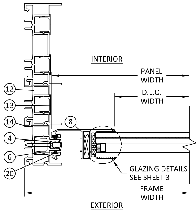
L 7 HORIZONTAL SECTION 4-TRACK JAMB FIXED PANEL
