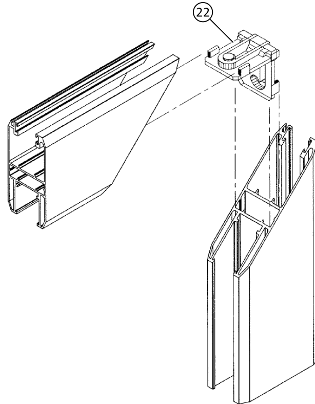
PANEL CORNER DETAIL
