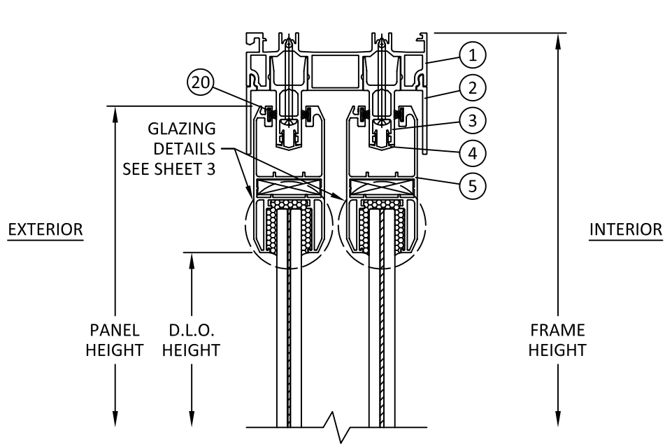
A 5 VERTICAL SECTION 2-TRACK HEAD
