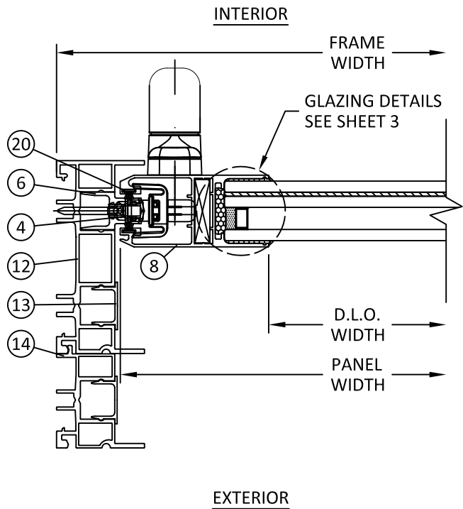
H 7 HORIZONTAL SECTION 3-TRACK JAMB OPERABLE PANEL
