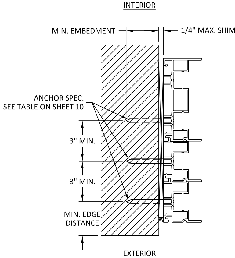
V 9 INSTALLATION DETAIL 4-TRACK JAMB
