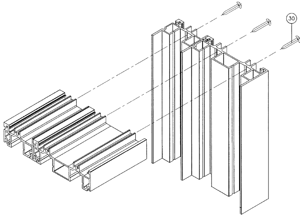
FRAME CORNER DETAIL 3 TRACK FRAME
