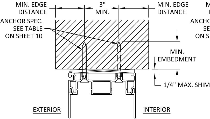
Q 9 INSTALLATION DETAIL 2-TRACK HEAD HEAD SHOWN, SILL SIMILAR
