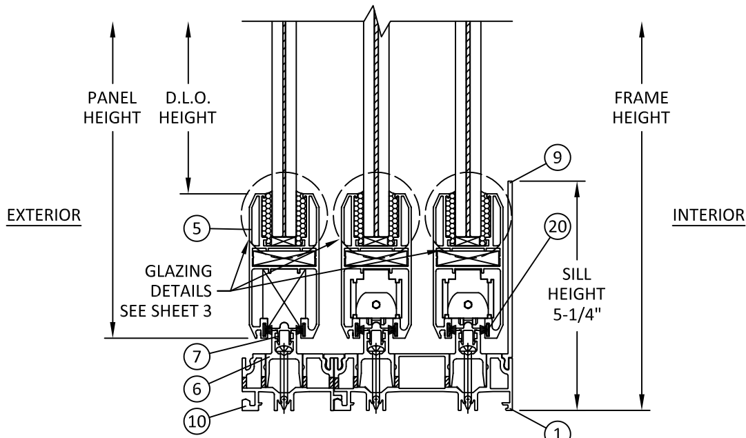
D 5 VERTICAL SECTION 3-TRACK SILL
