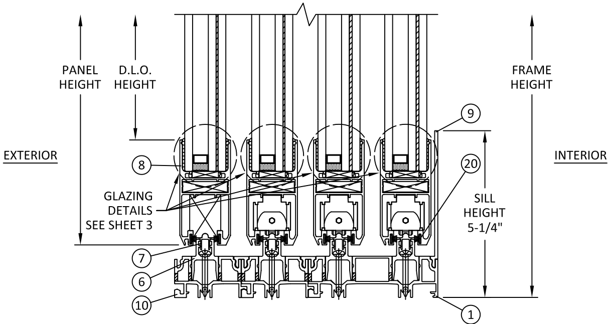
F 6 VERTICAL SECTION 4-TRACK SILL
