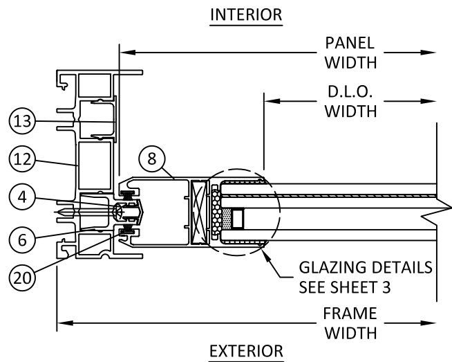
J 7 HORIZONTAL SECTION 2-TRACK JAMB FIXED PANEL
