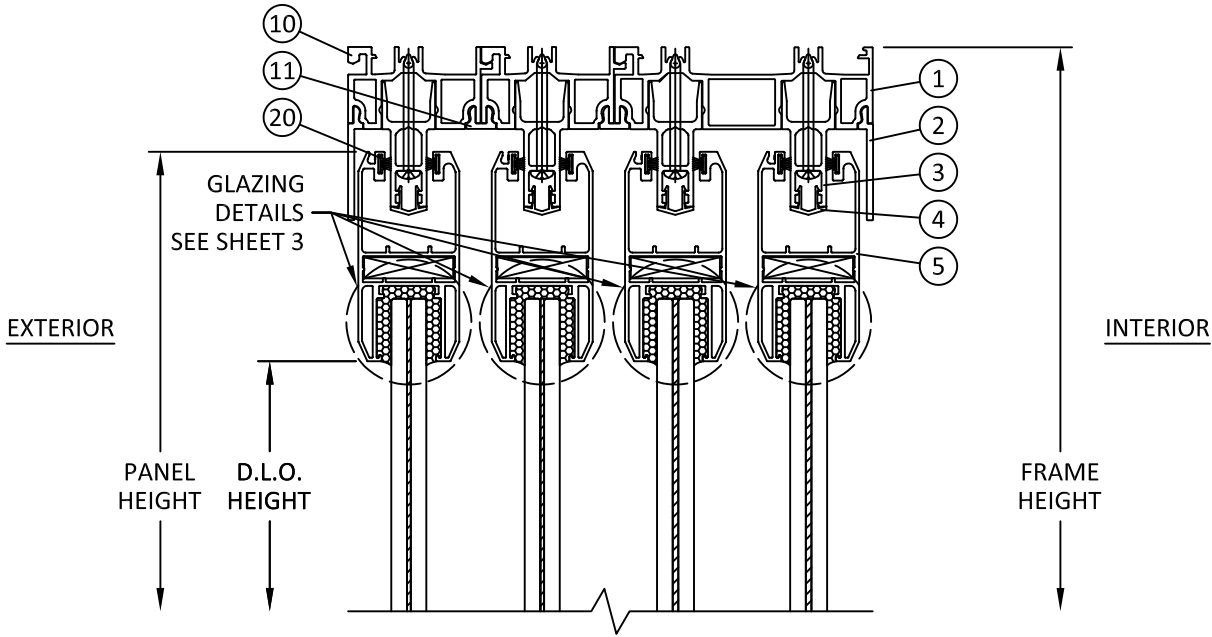
E 6 VERTICAL SECTION 4-TRACK HEAD
