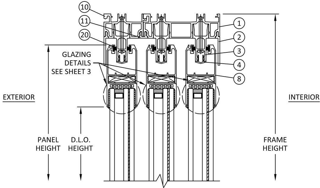
C 5 VERTICAL SECTION 3-TRACK HEAD
