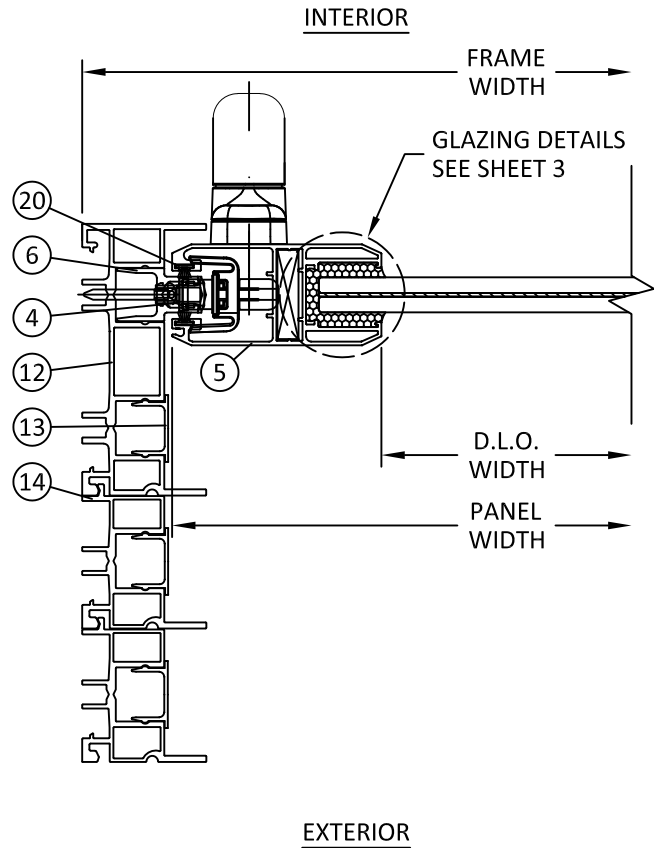
I 7 HORIZONTAL SECTION 4-TRACK JAMB OPERABLE PANEL
