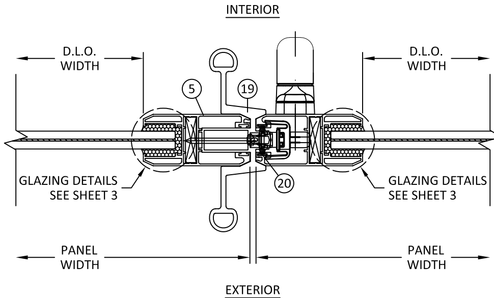
P 8 HORIZONTAL SECTION HD ASTRAGAL
