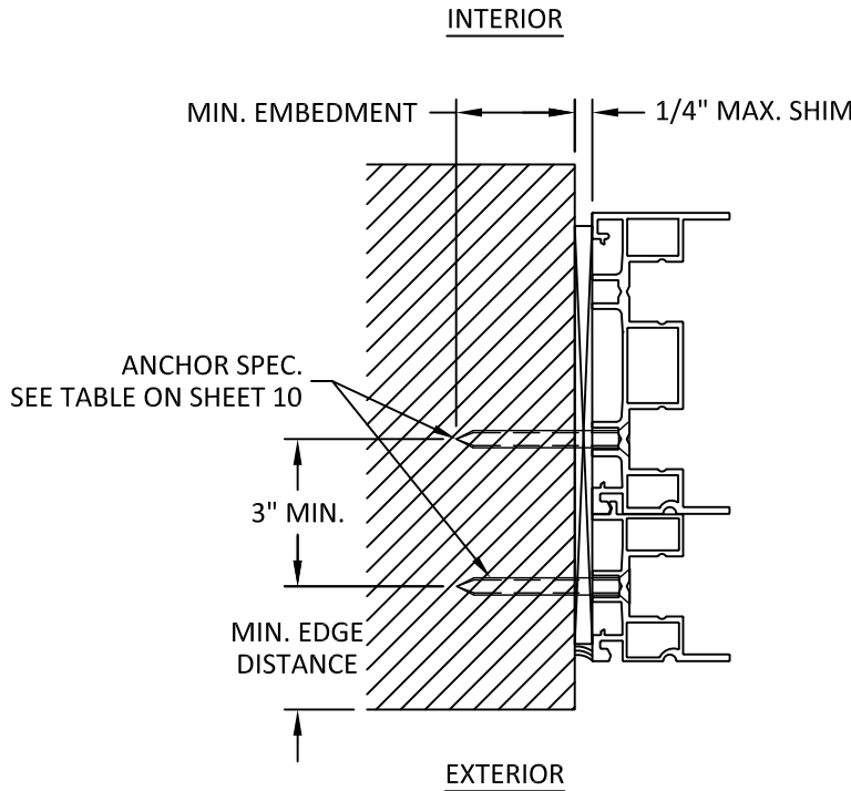
U 9 INSTALLATION DETAIL 3-TRACK JAMB
