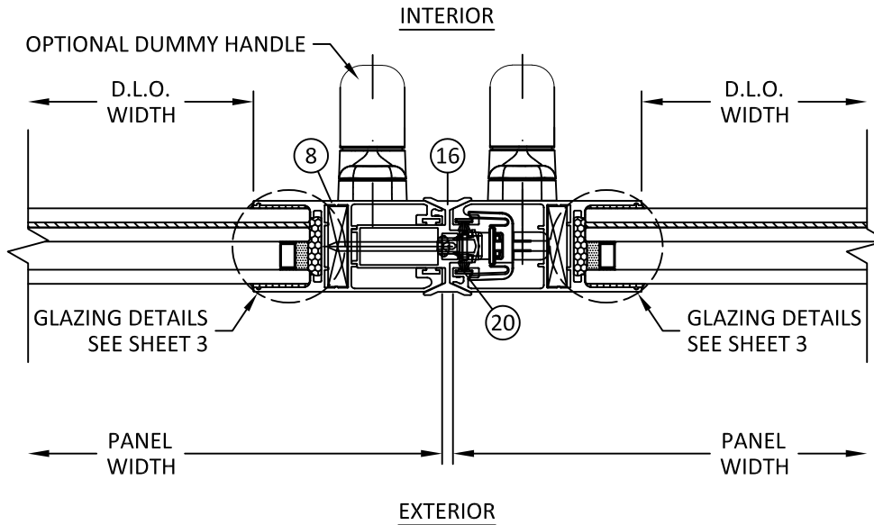
N 8 HORIZONTAL SECTION ASTRAGAL
