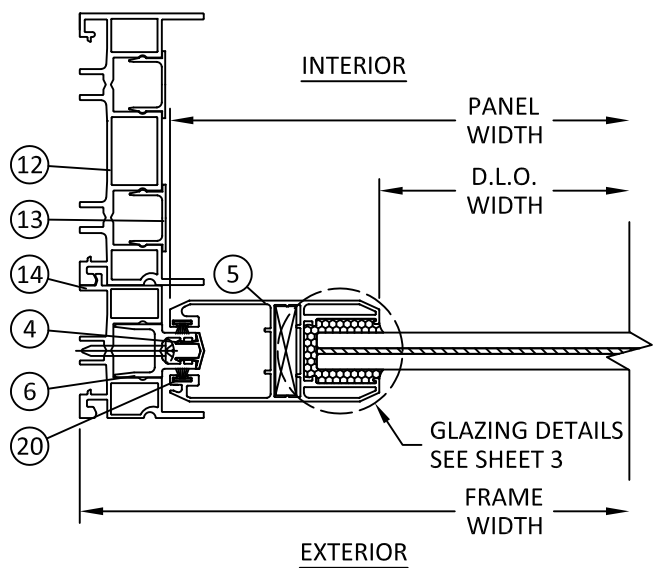
K 7 HORIZONTAL SECTION 3-TRACK JAMB FIXED PANEL
