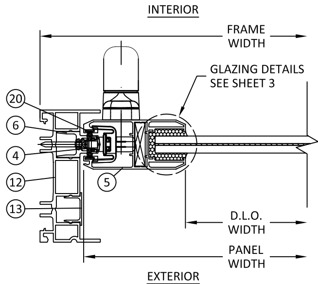
G 7 HORIZONTAL SECTION 2-TRACK JAMB OPERABLE PANEL
