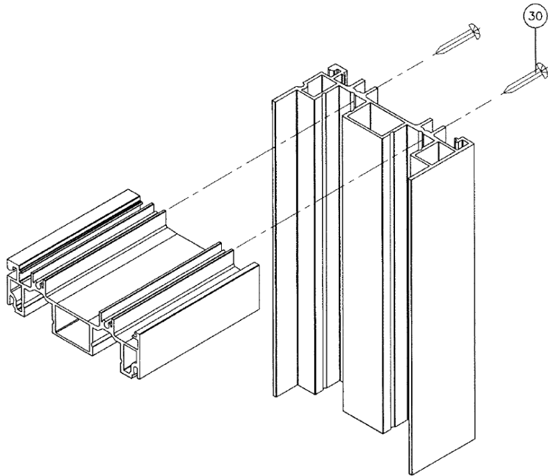
FRAME CORNER DETAIL 2 TRACK FRAME
