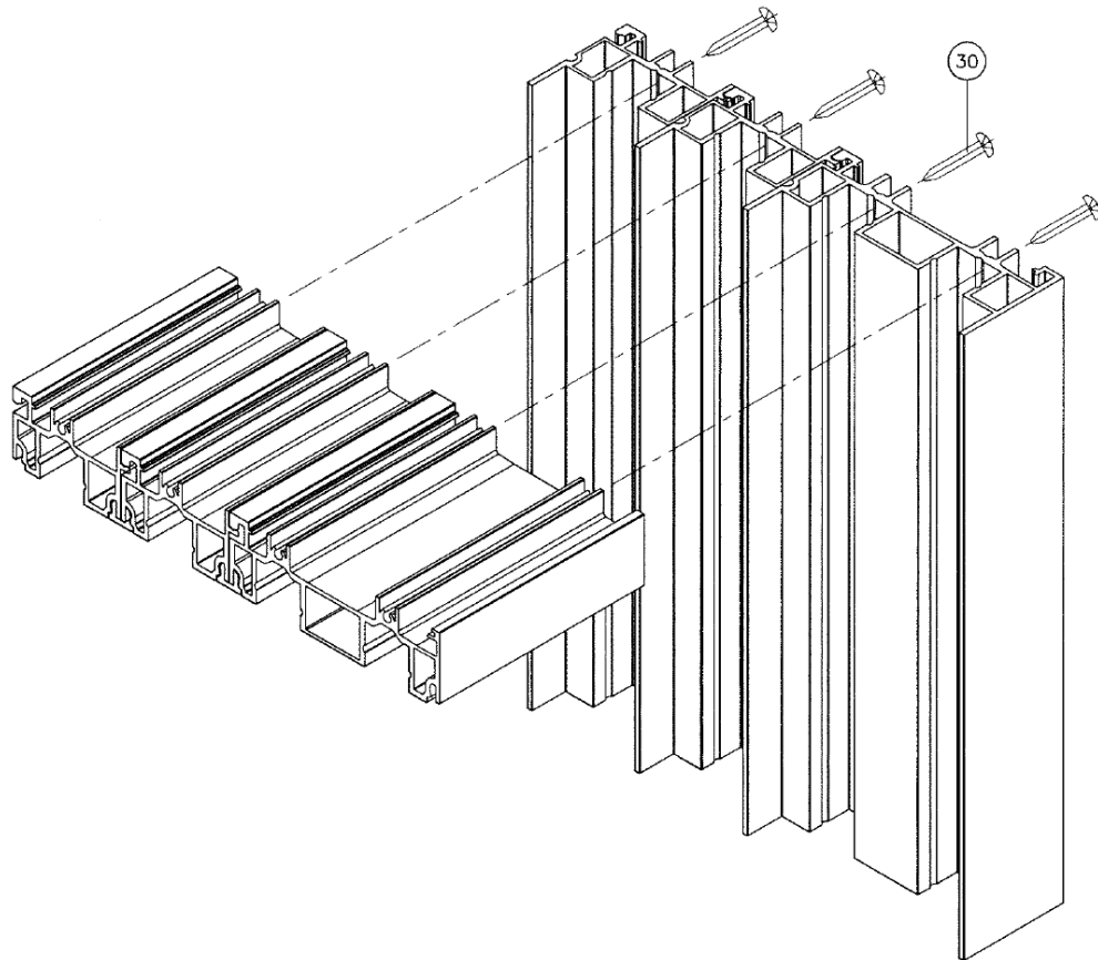
FRAME CORNER DETAIL 4 TRACK FRAME
